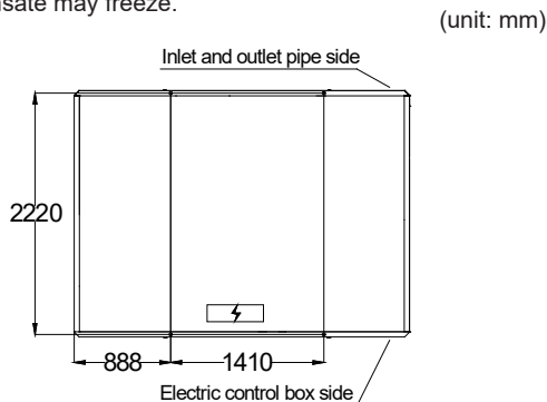
Fig. 6-6 Top view of schematic diagram of installation dimension of RHAH55/65/75HVN8H/E
