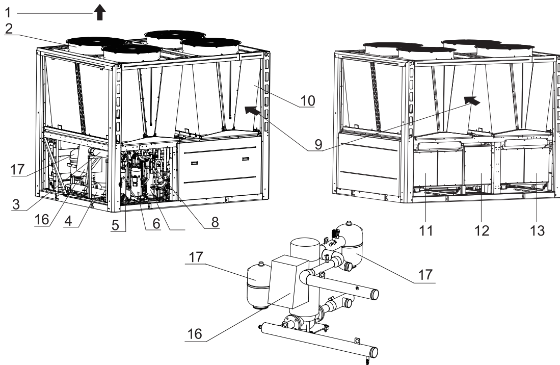
Fig. 8-1 Main parts of RHAH55/65/75HVN8H/E (Picture just use to show the key component relative position)
