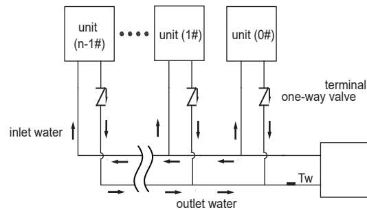
Fig.8-21 Installation of multiple water pump
