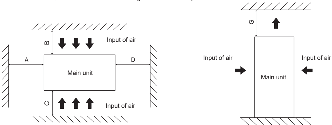
Fig. 6-3 single unit installation
