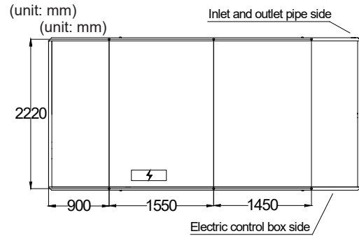
Fig. 6-7 Top view of schematic diagram of installation dimension of RHAH100/105/110HVN8H/E
