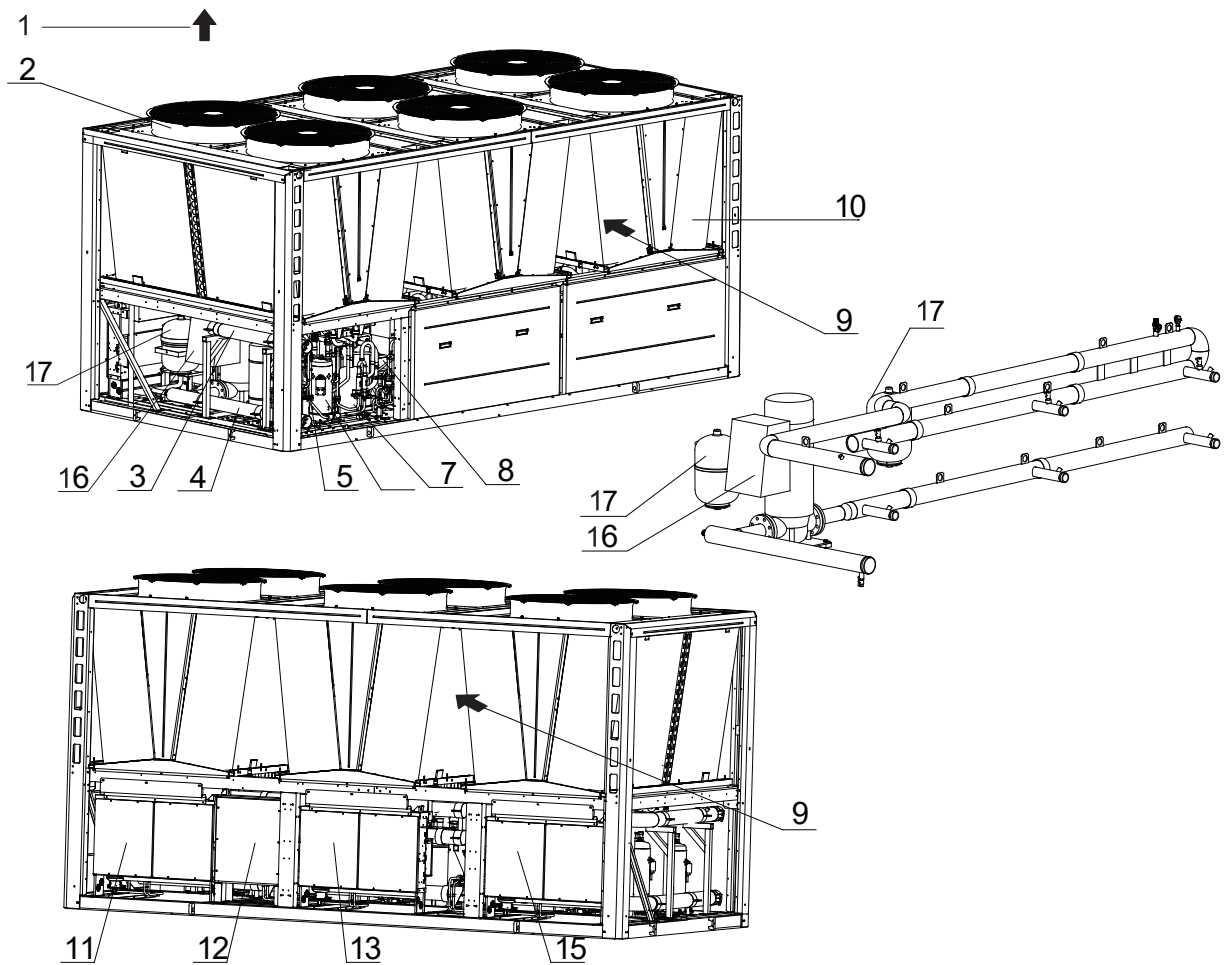
Fig. 8-1 Main parts of RHAH55/65/75HVN8H/E (Picture just use to show the key component relative position)
