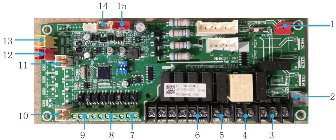
Fig. 8-6 Slave board
