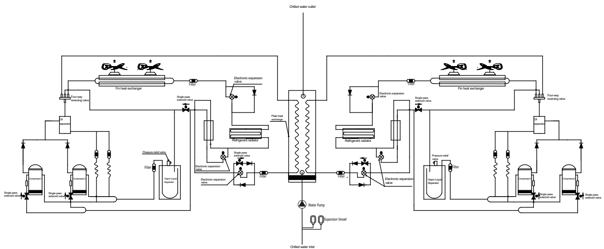
Fig. 6-1 Outline dimensional and system schematic diagram of RHAH55/65/75HNV8H/E
